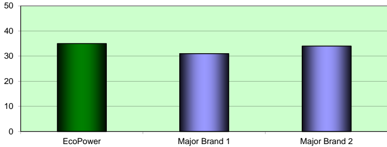
Iron (ppm per 10,000 miles)
